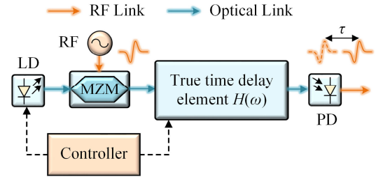
Fig. 4. Schematic of the typical optically-controlled true time delay system. MZM, Mach-Zehnder modulator.
