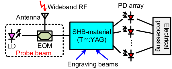
Fig. 13. Spectrum analyzer based on spatial-spectral material with an engraving laser. SHB: spectral hole burning.
