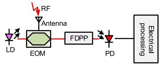
Fig. 15. Microwave frequency measurement system based on microwave power monitoring. FDPP: frequency-dependent power penalty.
