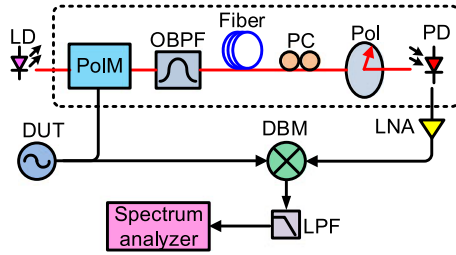
Fig. 5. Phase noise measurement system based on a microwave-photonic phase shifter. PoIM: polarization modulator. OBPF: optical band pass filter. PC: polarization controller. Pol: polarizer.
