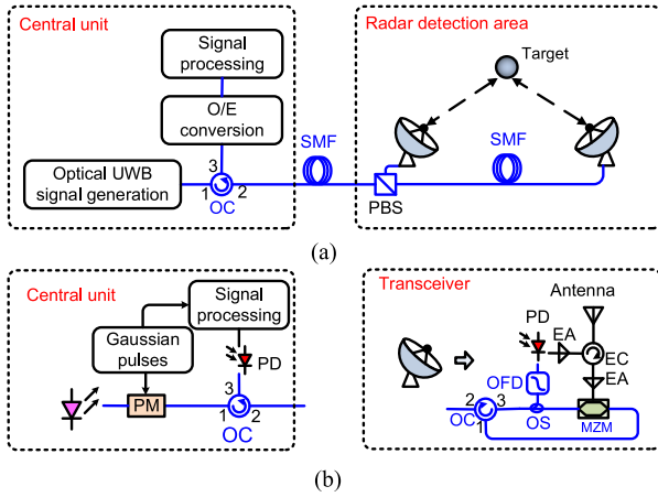
Fig. 23. Fiber-distributed UWB radar network based on wavelength reusing transceivers. OFD: optical frequency discriminator. EC: electrical circulator.
