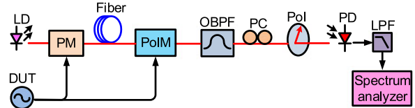
Fig. 7. Phase noise measurement system applying both microwave photonic phase shifter and microwave photonic down-converter.
