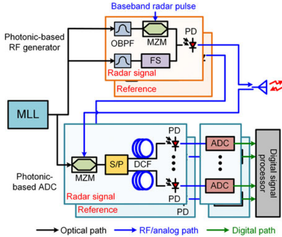
Fig. 20. Radar system based on photonic-based RF generator and photonic-based ADC. S/P: series-to-parallel converter. DCF: dispersion compensation fiber FS: frequency shifter.
