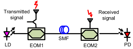
Fig. 26. Photonic Doppler frequency shift estimation system.
