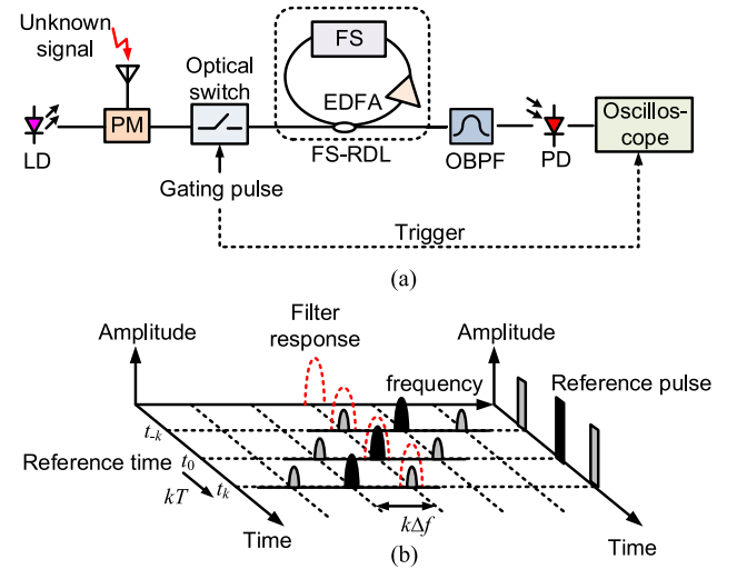
Fig. 18. Multiple-frequency measurement based on a FS-RDL. (a) Schematic diagram. (b) Operation principle. FS: frequency shifter. RDL: recirculating delay line.
