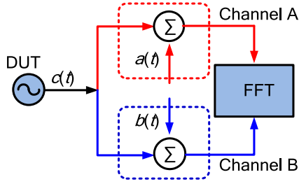
Fig. 8. Two-channel cross-correlation technique for phase noise measurement. FFT: fast Fourier transformation.
