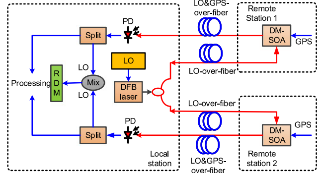
Fig. 27. Diagram of a typical multi-antenna based GPS positioning system. DM-SOA: directly modulated semiconductor optical amplifier. RDM: relative delay monitor.
