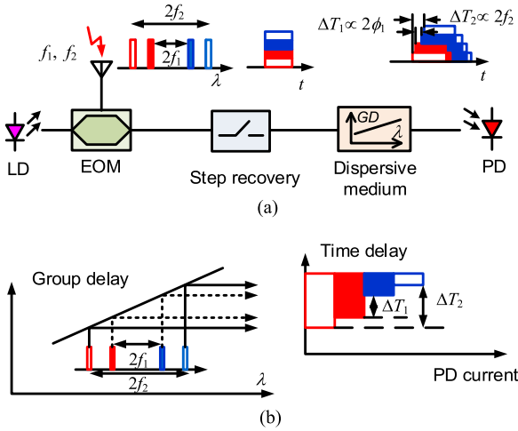
Fig. 17. Multiple-frequency measurement based on frequency-to-time mapping in a dispersive element. (a) Schematic diagram. (b) Operation principle.
