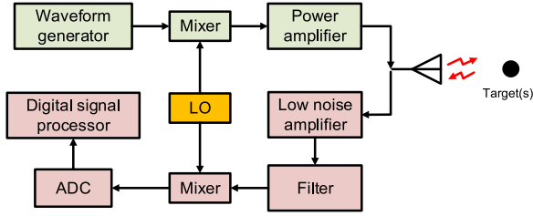
Fig. 19. Typical radar system. LO: local oscillator; ADC: analog-to-digital converter.
