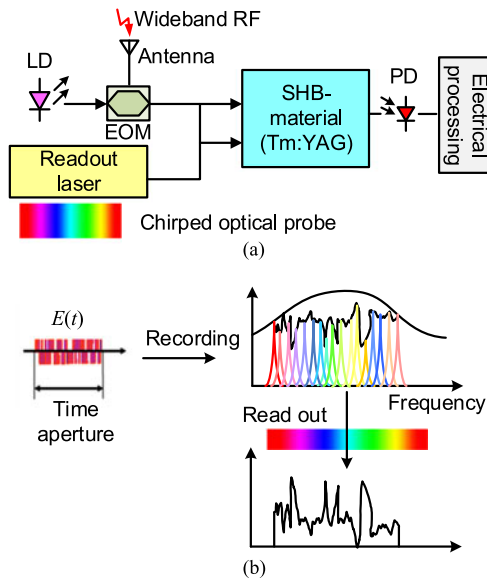
Fig. 14. Spatial-spectral material based spectrum analyzer with a linear chirped laser. (a) Schematic diagram. (b) Operation principle.
