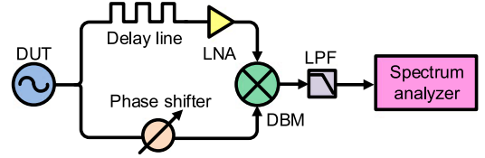
Fig. 3. Phase noise measurement system based on a frequency discriminator. DUT: device under test. LPF: low pass filter. LNA: low noise amplifier. DBM: double-balanced mixer.
