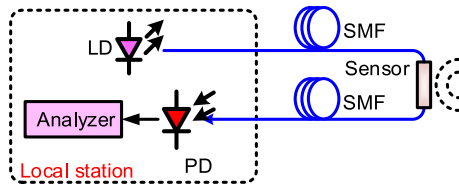
Fig. 2. Diagram of a typical electric-field measurement system. LD: laser diode. PD: photodetector. SMF: single mode fiber.
