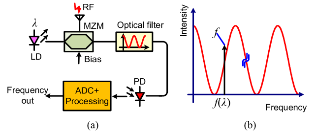
Fig. 16. Microwave frequency measurement system based on optical power monitoring. (a) Schematic diagram. (b) Operation principle.
