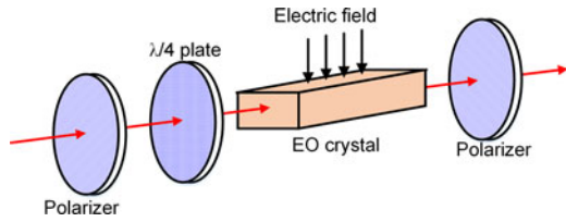
Fig. 1. Diagram of a typical electric-optic sensor. EO crystal: electro-optic crystal.
