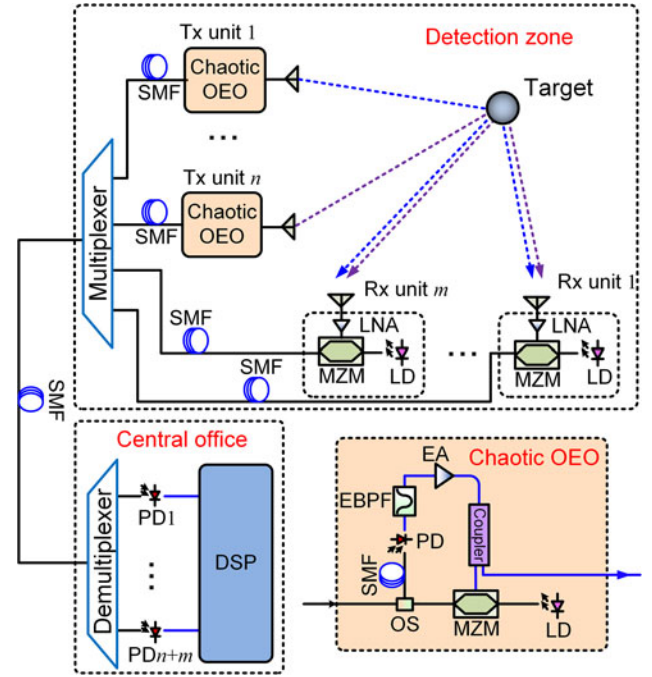
Fig. 24. Distributed MIMO chaotic radar based on WDM technology. OS: optical splitter. EBP: electrical bandpass filter. EA: electrical amplifier.
