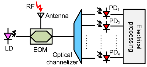
Fig. 10. Microwave spectrum analysis system based on an optical channelizer. EOM: electro-optical modulator.
