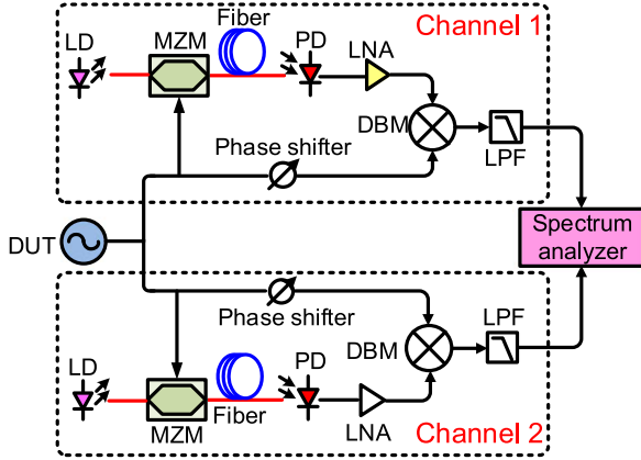
Fig. 9. Two-channel cross-correlation system based on optical delay lines.
