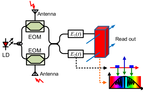
Fig. 25. DOA estimation system based on SHB effect.
