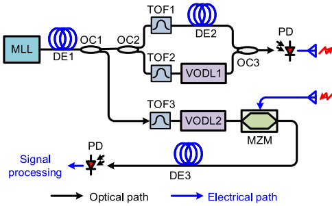
Fig. 21. Photonics-based radar system in [87]. DE: dispersion element; OC: optical coupler; TOF: tunable optical filter; VODL: variable optical delay line.
