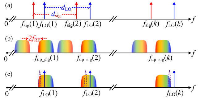
Fig. 12. Optical channelization based on dual coherent OFCs. (a) The signal OFC and local OFC. (b) The modulated signal OFC. (c) Extracting different spectrum slices of the microwave signal in each channel. OFC: OFC.
