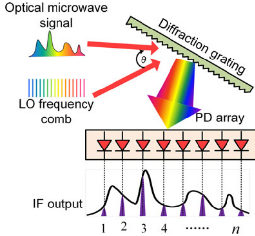
Fig. 11. Diagram of the microwave spectrum analysis system based on coherent optical channelizer using a diffraction grating.
