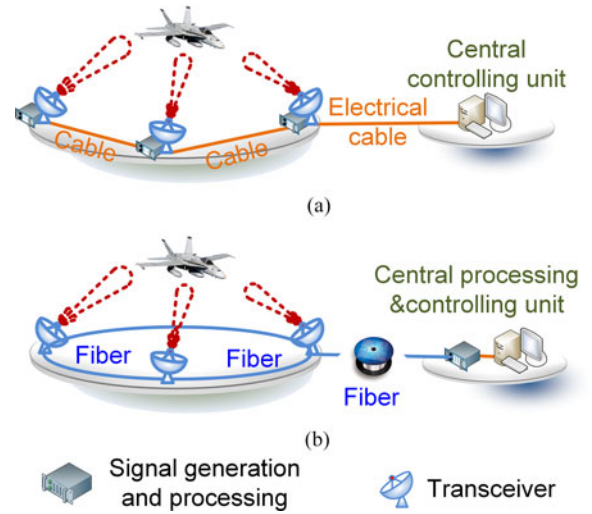
Fig. 22. (a) Conventional distributed radar system. (b) Fiber-connected distributed radar system.
