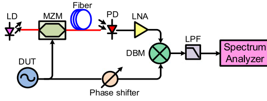
Fig. 4. Phase noise measurement system based on optical fiber delay. MZM: Mach-Zehnder modulator.
