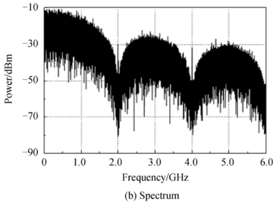
图2 PRBS 信号的眼图和频谱 Fig.2 The eye diagram and spectrum of the PRBS signal
