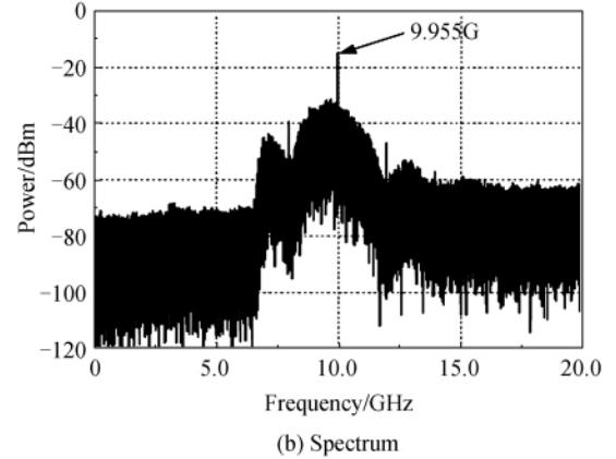
图4 天线接收信号的眼图和频谱 Fig.4 The eye diagram and spectrum of the signal received by antenna
