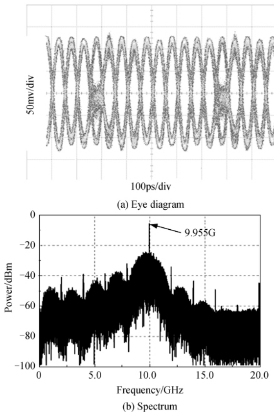
图3 PRBS 信号上转换后的眼图和频谱 Fig.3 The eye diagram and spectrum of the upconverted PRBS signal
