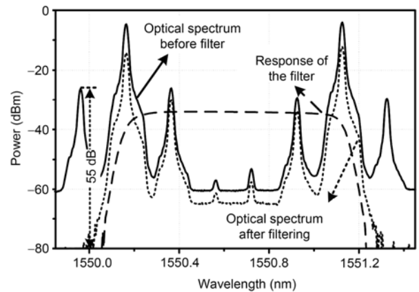
Figure 2 The optical spectra of the signals before and after the OBPF, and the transmission response of the OBPF.
