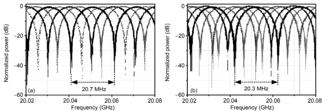
Figure 5 Frequency responses of the MPF with one DSB tap and (a) 25-km SMF transmission and (b) 40-km SMF transmission.
