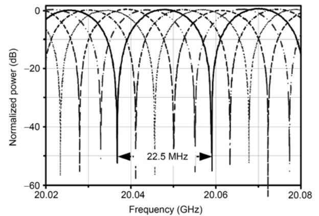
Figure 3 The measured frequency response of the proposed filter.
