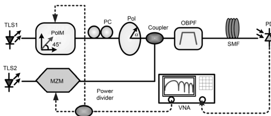
Figure 1 The schematic of the proposed microwave photonic filter. TLS: tunable laser source; PC: polarization controller; PolM: polarization modulator; SMF: single mode fiber; PBS polarization beam splitter; PD: photodetector; VNA: vector network analyzer; MZM: Mach-Zehnder modulator.
