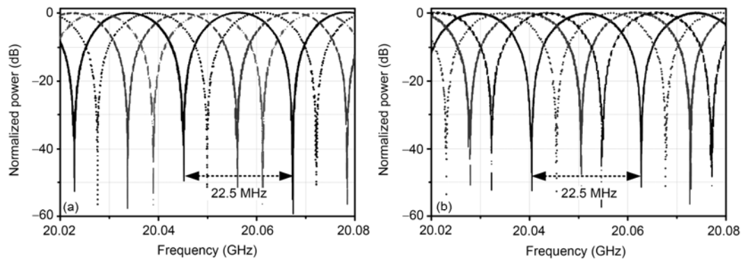
Figure 4 Frequency responses of the proposed MPF with (a) 25-km SMF transmission and (b) 40-km SMF transmission.
